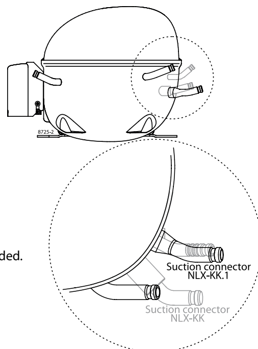
fig. Connector positions on NLX-KK compressor (grey) and NLX-KK.1 compressor (black).
